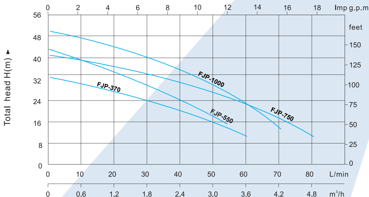
PERFORMANCE CHART AT n=2900 r/min
